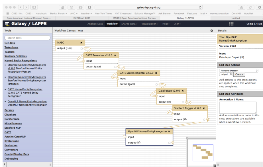
Fig. 4: The LAPPS/Galaxy Interface: Workflow configuration
