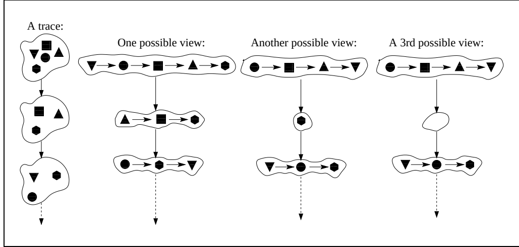
Figure 3.2: paraDOS Concepts: trace and views.
