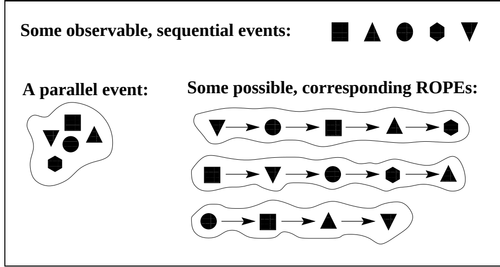
Figure 3.1: paraDOS Concepts: events, parallel event, and ROPEs.
