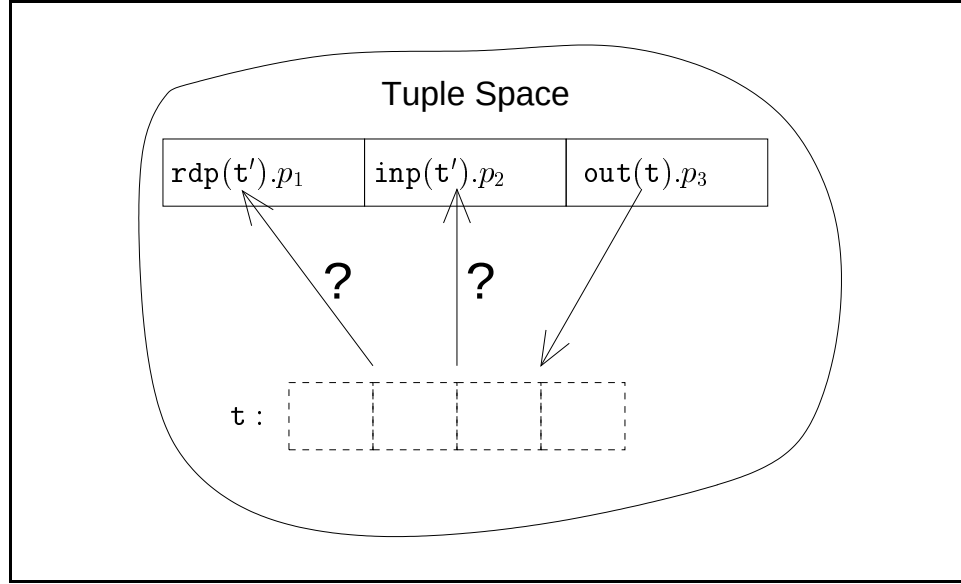
Figure 9.1: Case Study for Linda predicate ambiguity: an interaction point in tuple space involving three processes.
