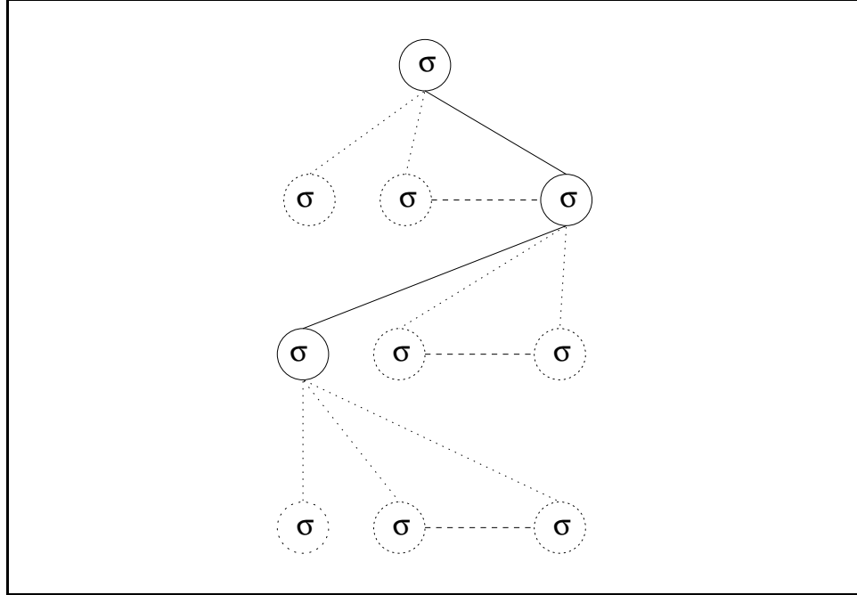
Figure 3.3: ParaDOS computation space: a lazy tree.
