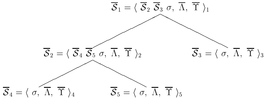
Figure 8.2: Example composition tree from derivation of \overline{\mathcal{S}}
