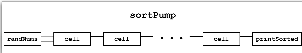
Figure 1: Process network for a sortPump. Two channels connecting each pair of processes—one to pass numbers being sorted, and the other a kill channel. There are as many cell processes as random numbers being sorted.
